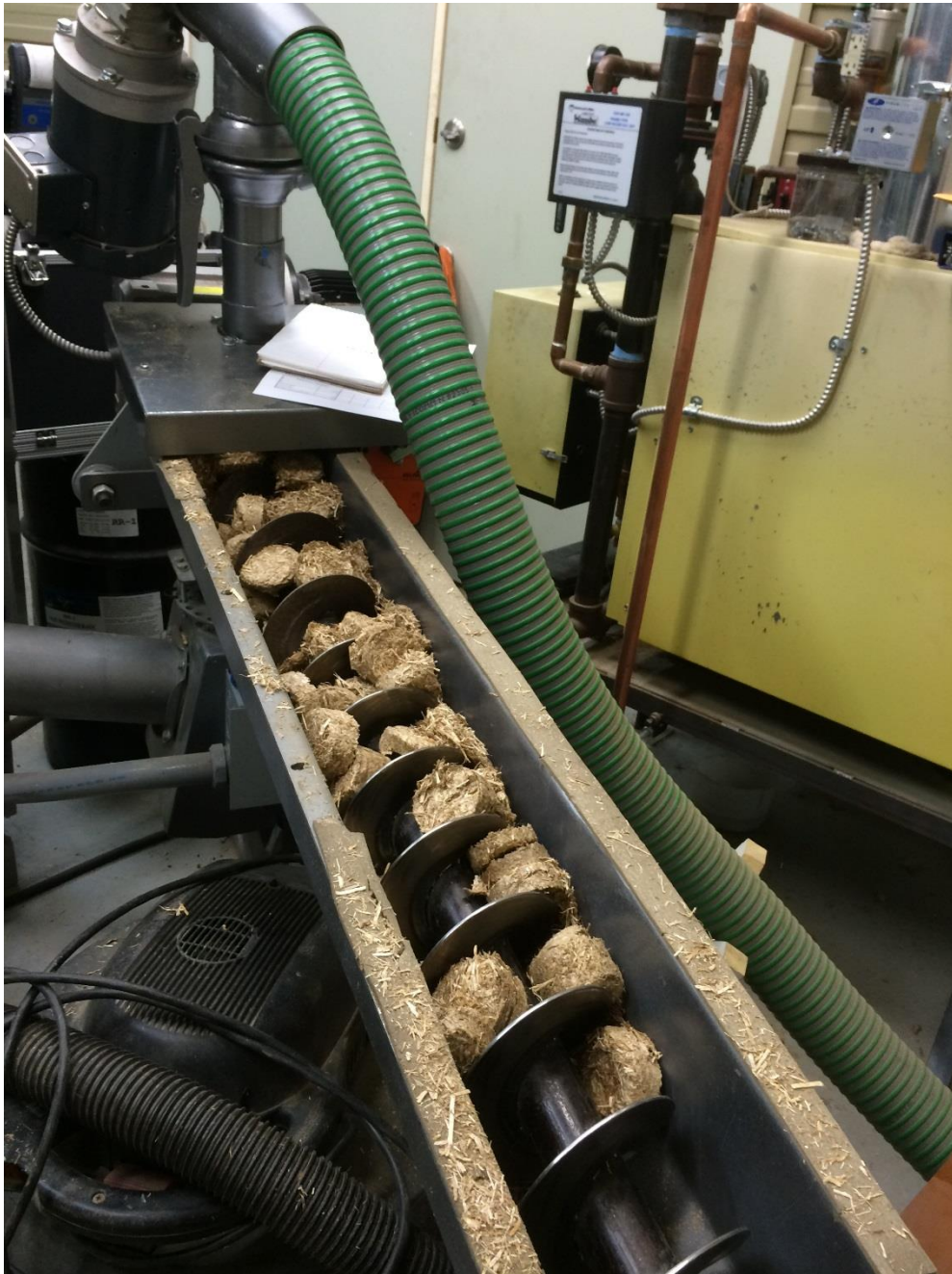
Figure 6 - The primary feed auger on the EvoWorld HC100. The green tube is a parallel wood pellet feed system. Both of these systems feed into a "hand off box" below where they join. The combustion feeder moves fuel from the hand off box to the combustion chamber. The hand-off box has a fire damper to separate the combustion area from the primary feed (and fuel storage) area.
