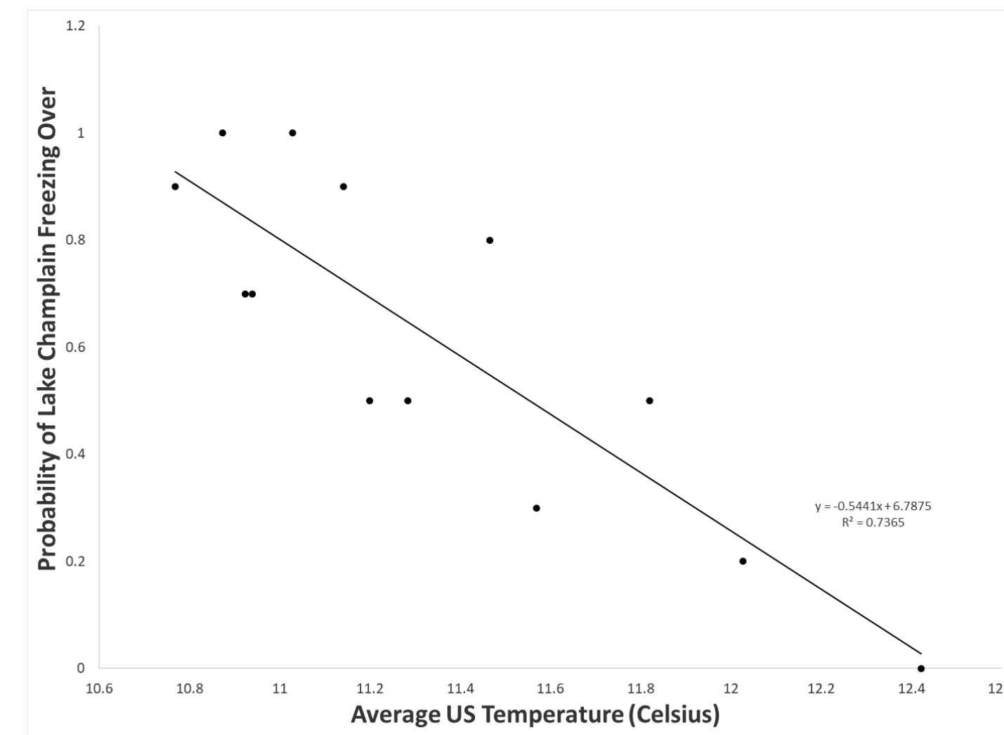
Figure 3: The probability (out of 1) Lake Champlain will freeze over given mean US temperatures (Celsius)
